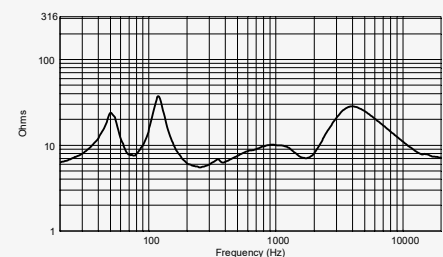
IMPEDANCE
