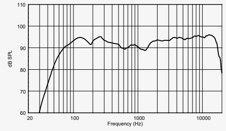
RESPONSE 1W/1m
