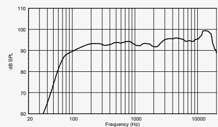
RESPONSE 1W/1m
