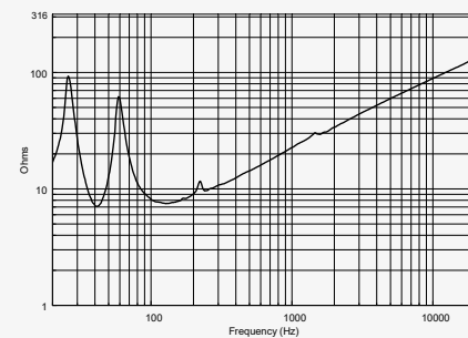
IMPEDANCE
